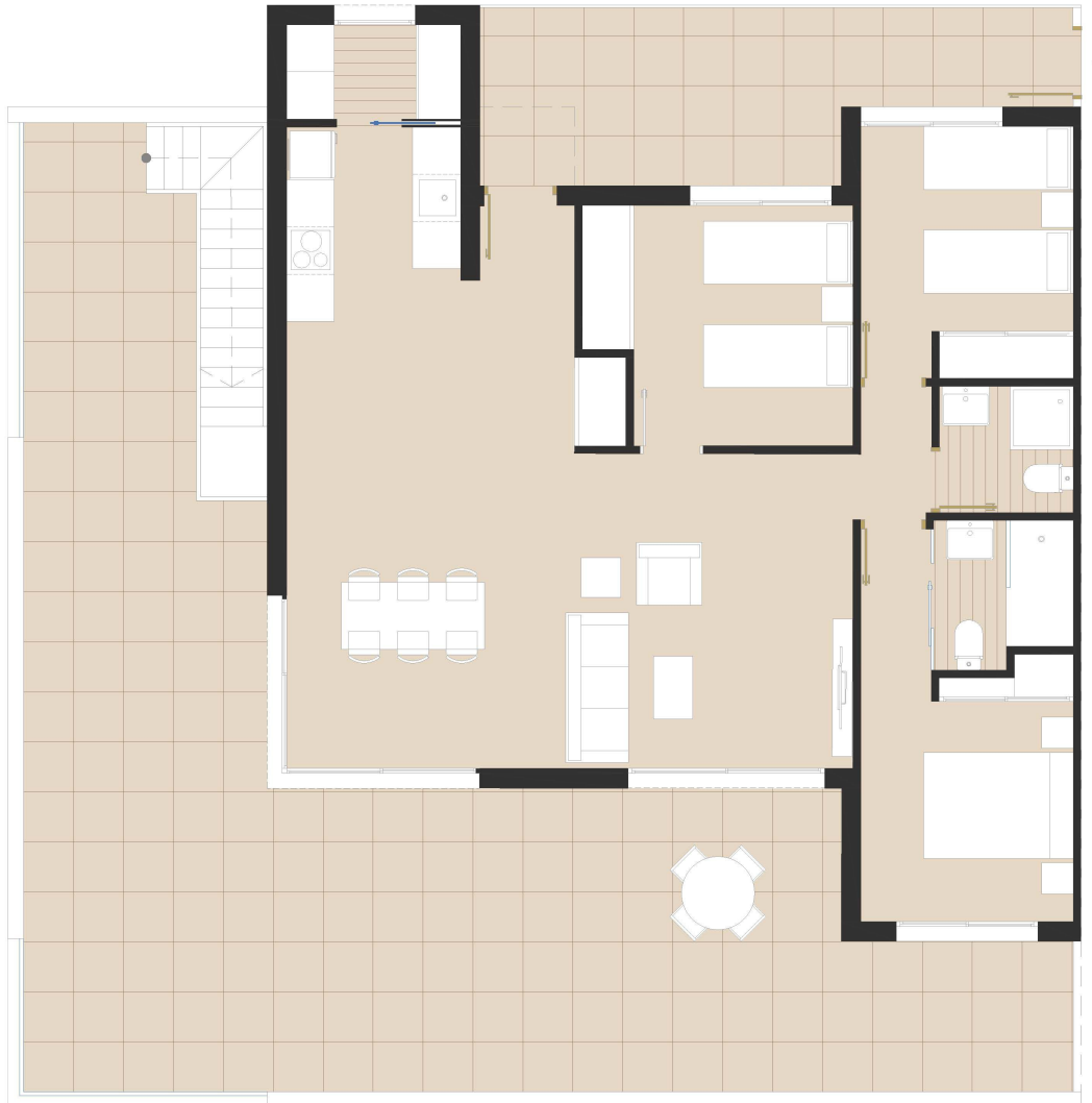
Second Floor/ Planta Segunda (E:1/100)
