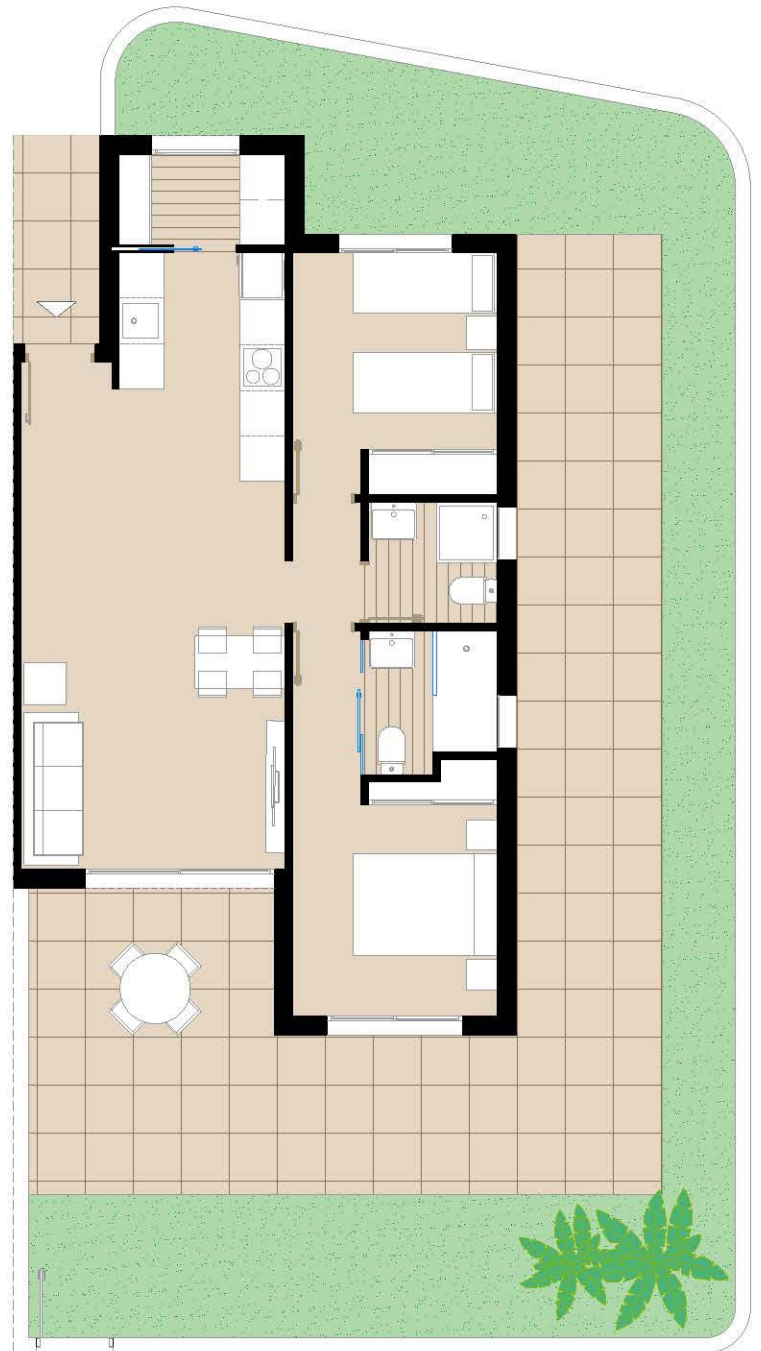
Ground Floor/ Planta Baja (E:1/100)
