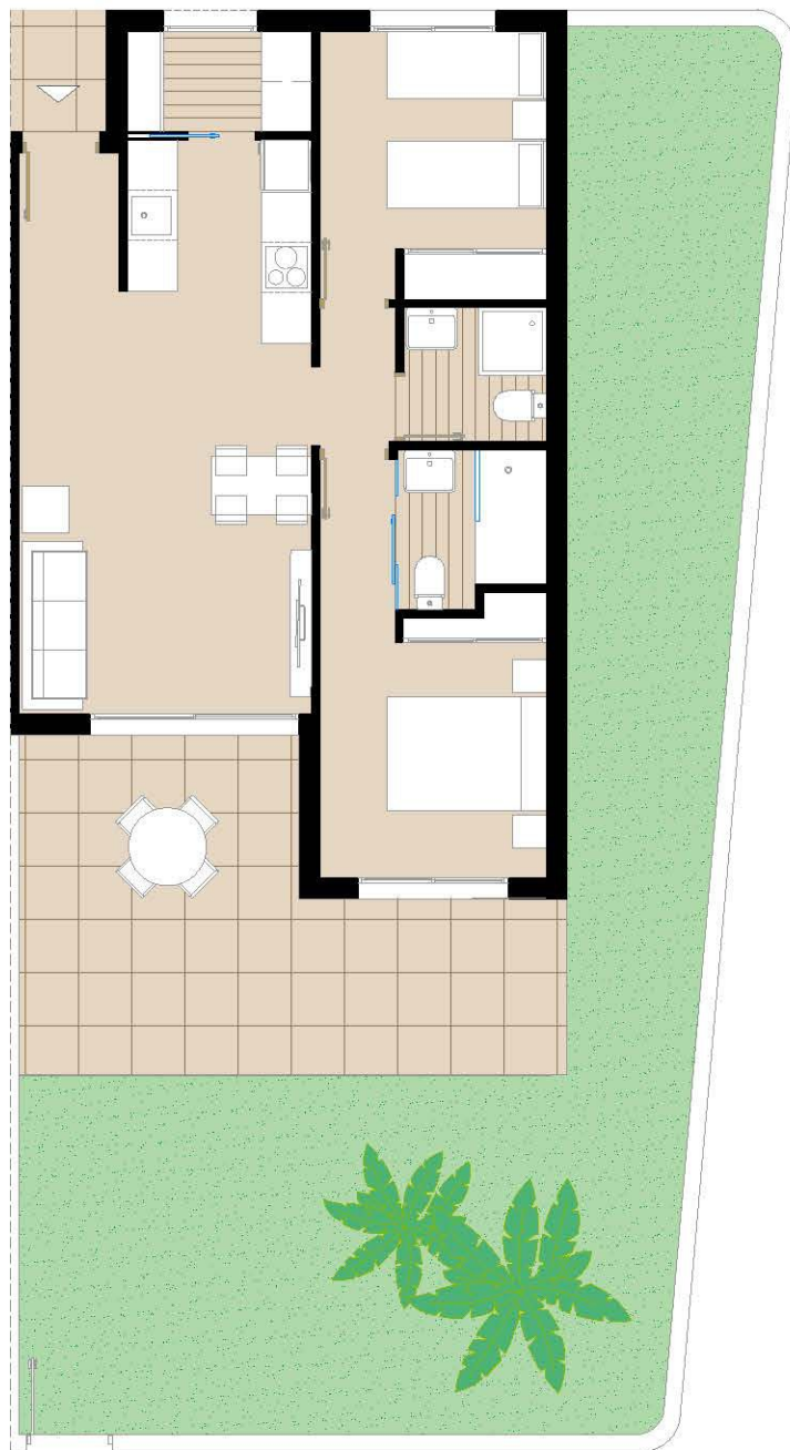
Ground Floor/ Planta Baja (E:1/100)
